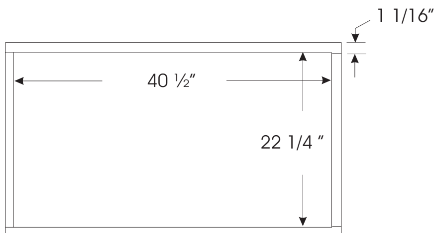
Inside frame dimensions - Top view
