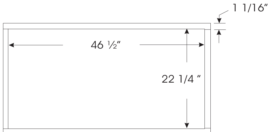
Inside frame dimensions - Top view
