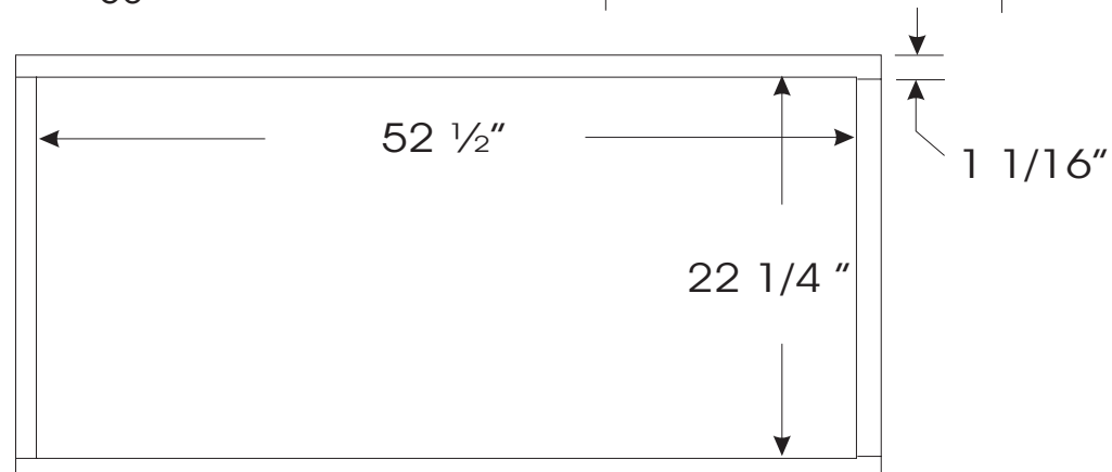
Inside frame dimensions - Top view
