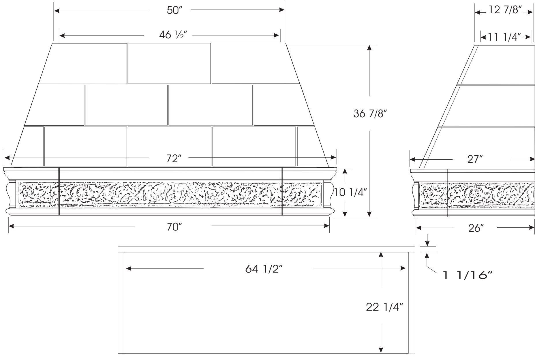
Inside frame dimensions - Top view
